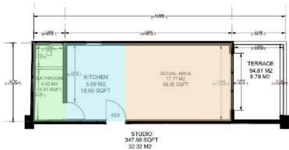
APARTMENT 404 ESC: 1:50
