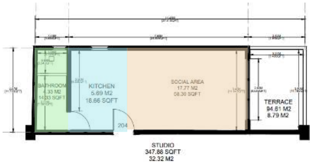
APARTMENT 204 ESC: 1:50
