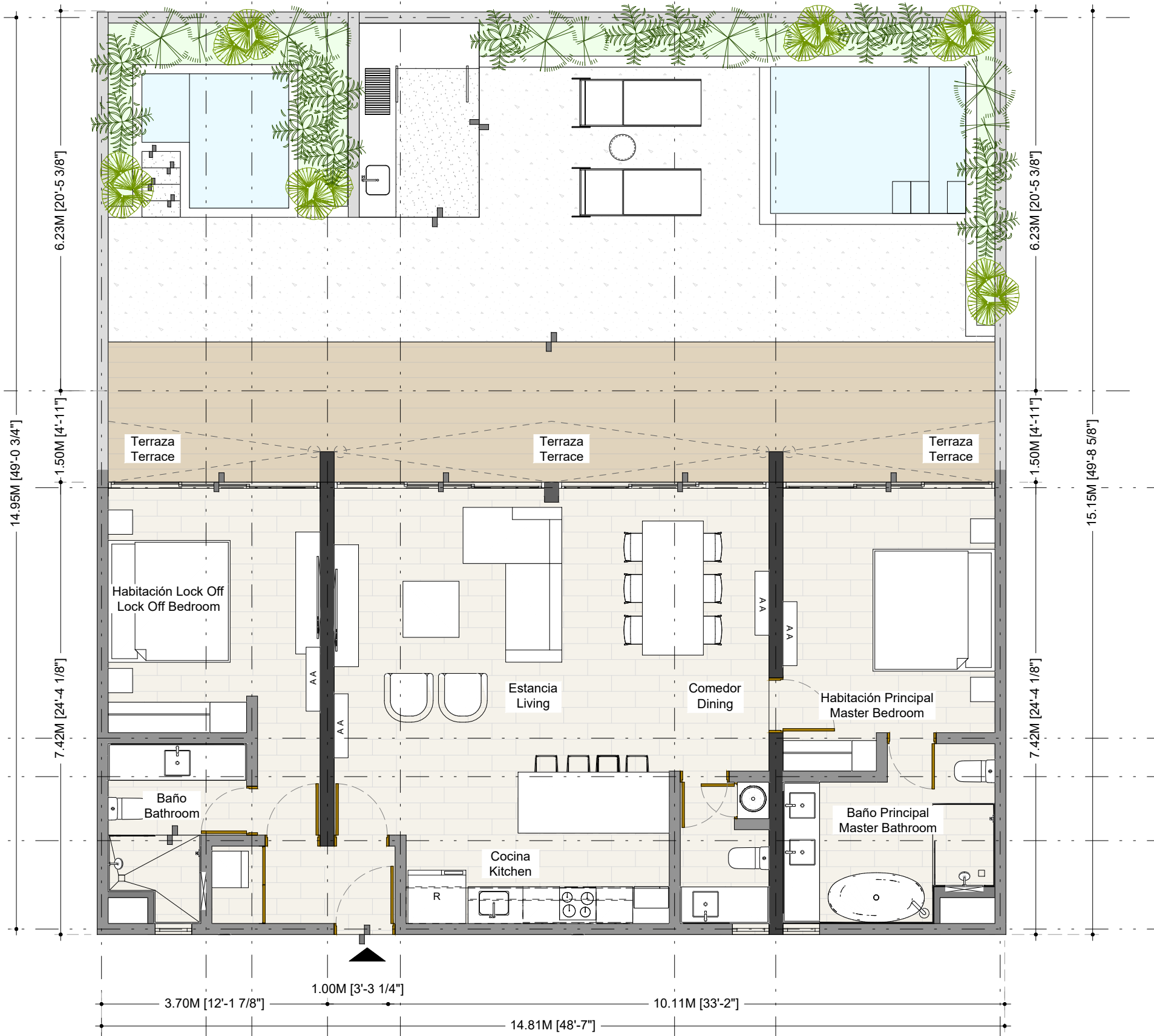
01 PLANTA ARQUITECTÓNICA - 2BR GARDEN POOL ARCHITECTURAL PLAN - 2BR GARDEN POOL
