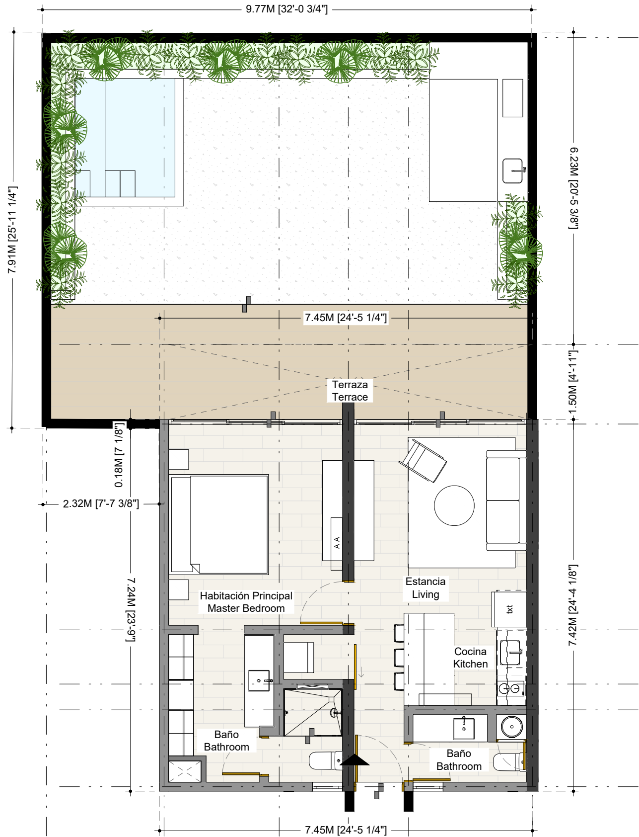
01 PLANTA ARQUITECTÓNICA - 1BR GARDEN POOL ARCHITECTURAL PLAN - 1BR GARDEN POOL
