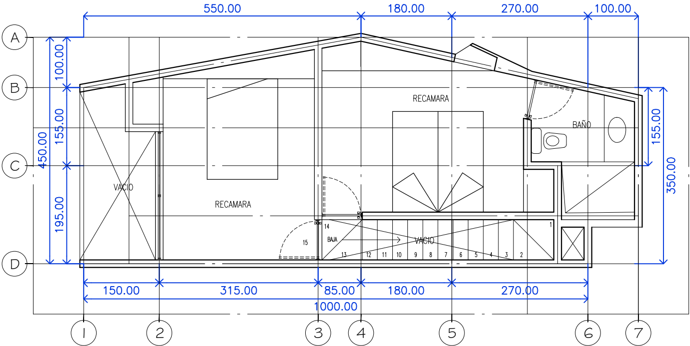
MEZANINE AREAS INTERIOR 36.4 M2 EXTERIOR 0 M2
