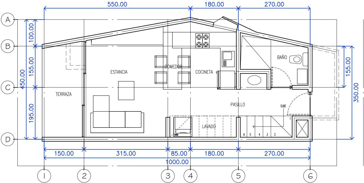
PLANTA BAJA AREAS INTERIOR 36.4 M2 EXTERIOR 5.6 M2
