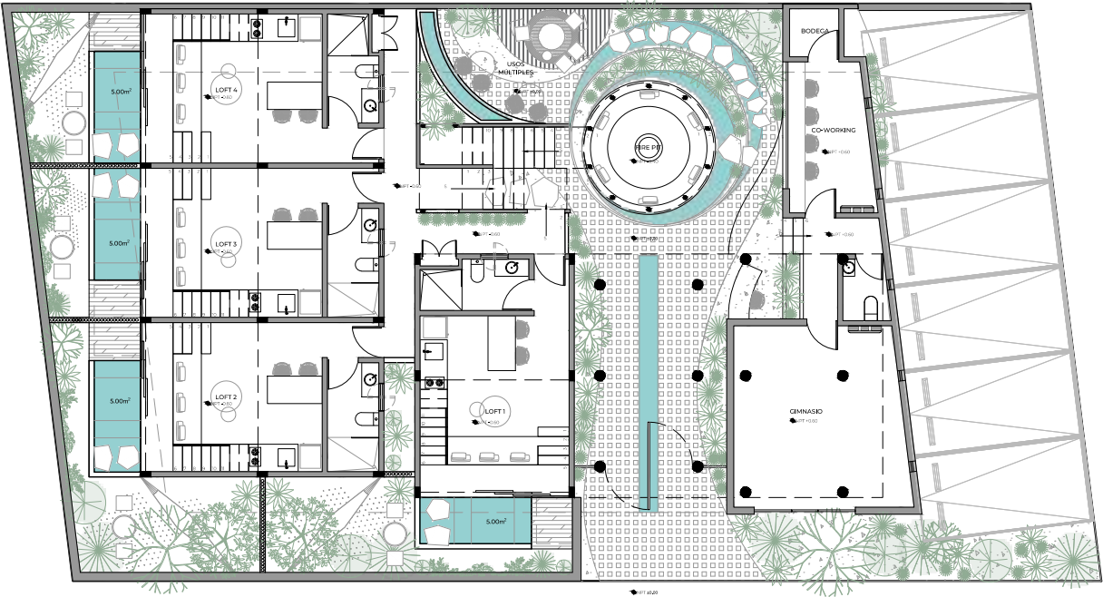
GROUND FLOOR GOLD GARDEN FLOORPLAN SCALE 1:200
