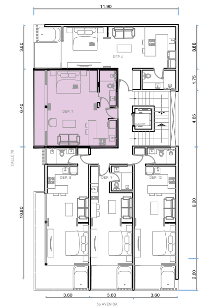
2nd LEVEL
